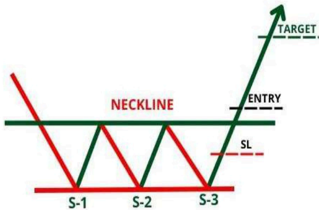
Triple Bottom
